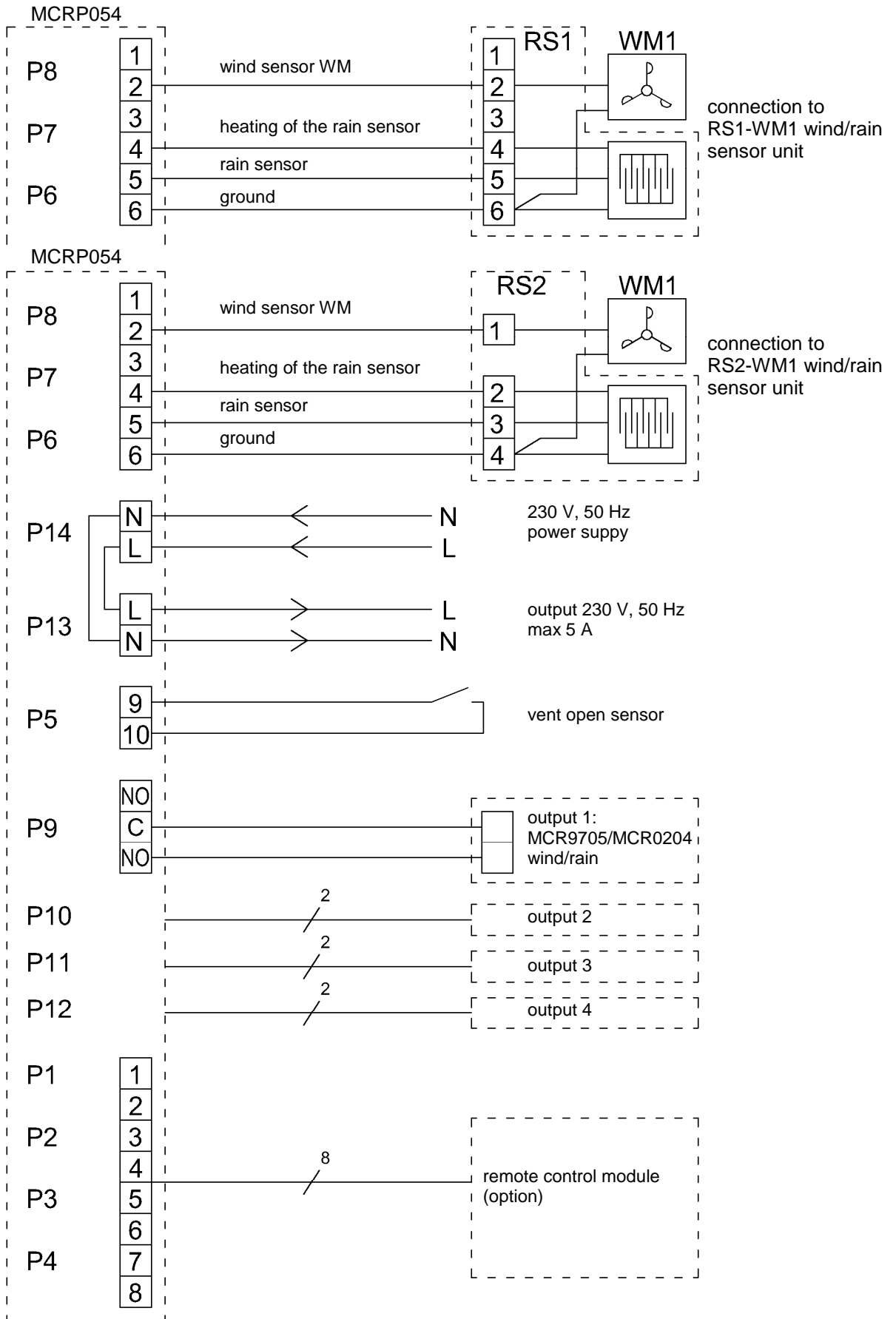
Drawing 1. Connection for the MCRP 054 weather monitoring unit with a RS2-WM1 sensor .
